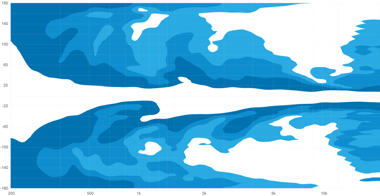
CARYS C6 Vertical beamwidth
